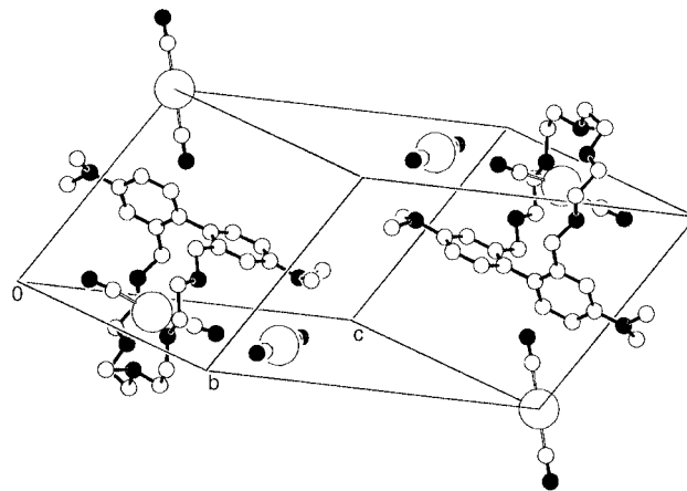
Fig. 2 View of molecular structure for [\text{HgL}^2(\text{CN})_2] \cdot 2\text{Hg}(\text{CN})_2 .
