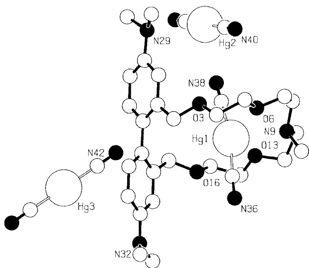
Fig. 1 Molecular structure with crystallographic numbering scheme for [\text{HgL}^2(\text{CN})_2] \cdot 2\text{Hg}(\text{CN})_2 . Hydrogen atoms have been omitted for clarity.
